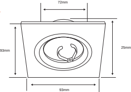
YD-620/AL BALME I
