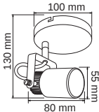
LVCLED-8401/6W/30S BOSSASO I
