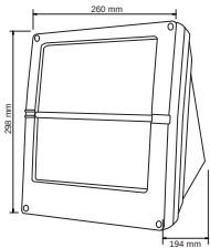
ES-5201 BURGOS Powered by PHILIPS
