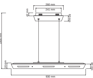
CTLLLED-160/27W/30 LIBERIA I
