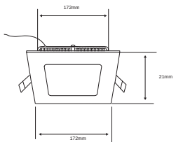
NUEVO YDLED-431/12W/30/B BRIGHTON I
