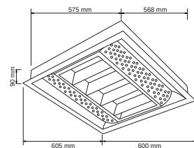
LTL-4140 MONDELLO 41: BLANCO FRÍO 65: LUZ DE DÍA Powered by PHILIPS
